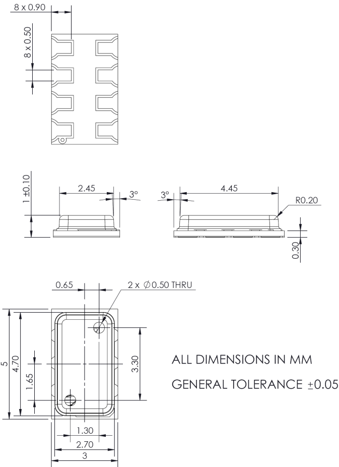
Figure 18: MS5607-02BA package outline
