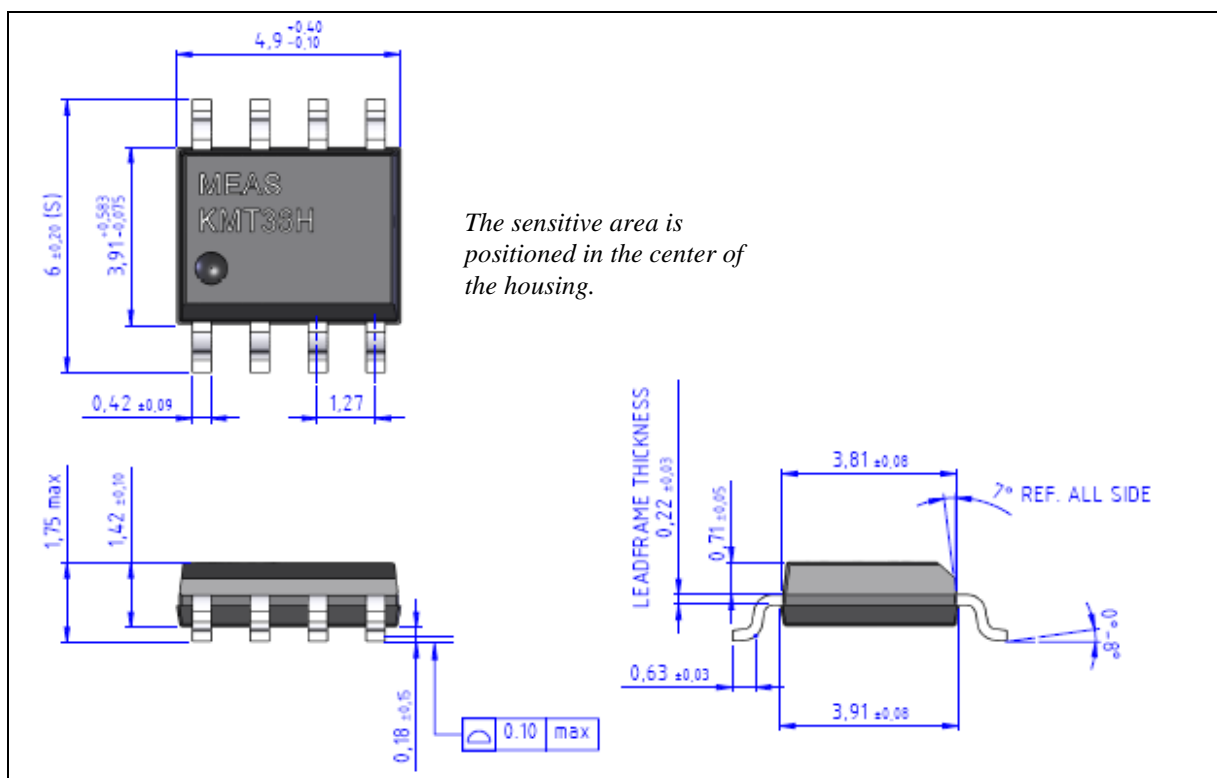
Figure 2: SO8 outline
