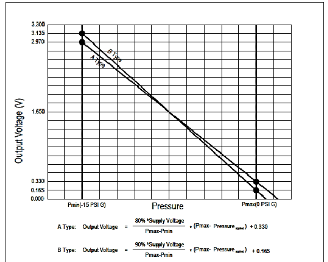
Vacuum Series Transfer Functions, Supply=3.3V
