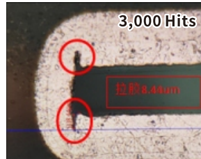
3,000 Hits Cross-Section 8.44 \mu m protrusion 3,000孔后切片 拉胶 8.44 \mu m
