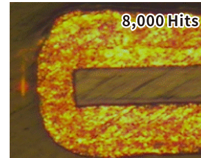
8,000 Hits Cross-Section no protrusion 8,000孔后切片 没出现 拉胶
